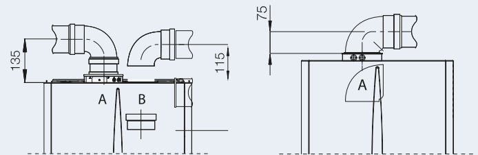
Kit double tuyau Ø 80/80
